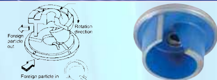
Single channel, semi-open impeller with tungsten cutting tip
