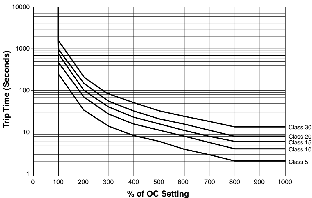
Figure 4: Overload Trip Curves
