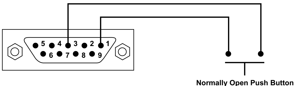
Figure 5: Remote Reset Button Wiring Diagram
