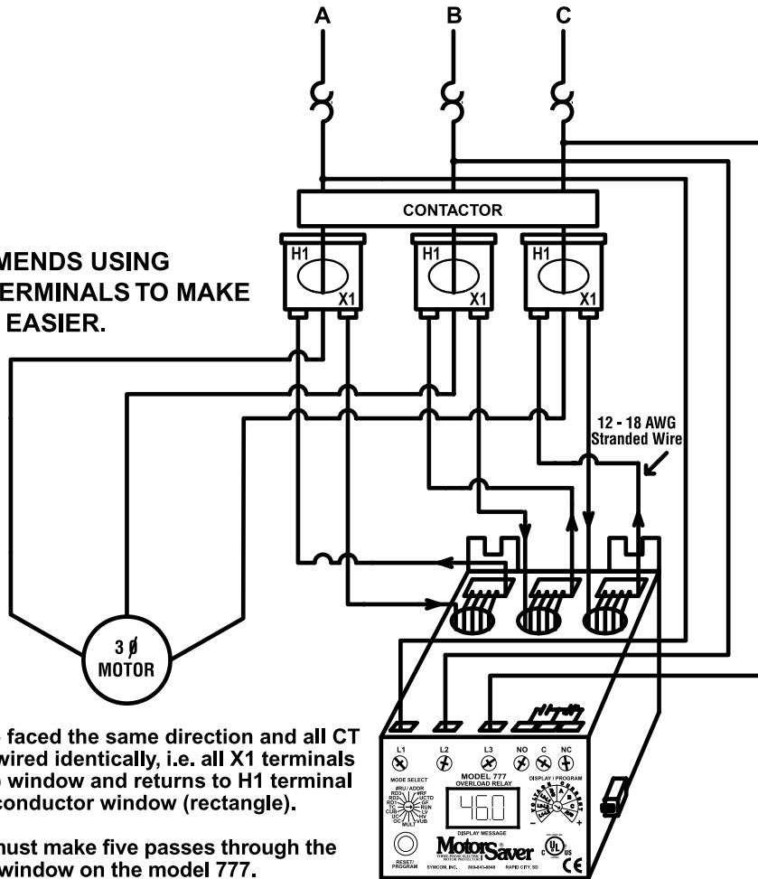
Figure 2: Typical Wiring Diagram Using External CTs.
