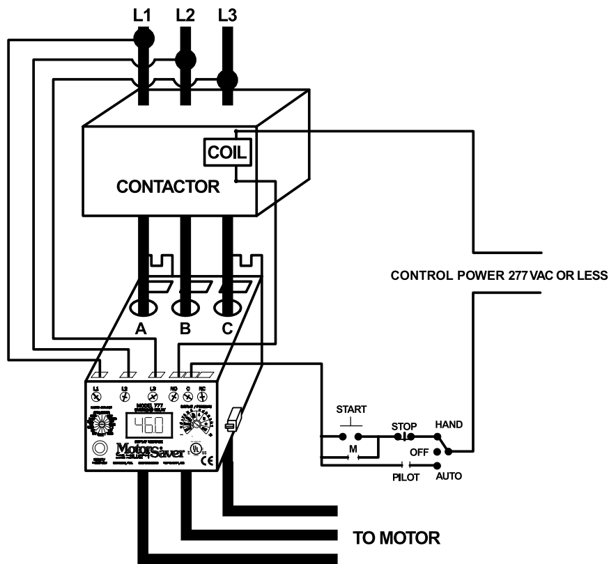
Figure 1: Typical Wiring Diagram for FLA of 26-90
